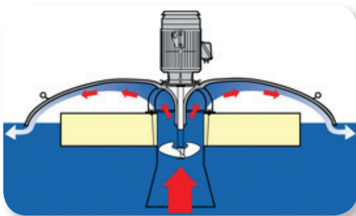
Illustration of the Aqua-Jet II® cover assembly operation.
